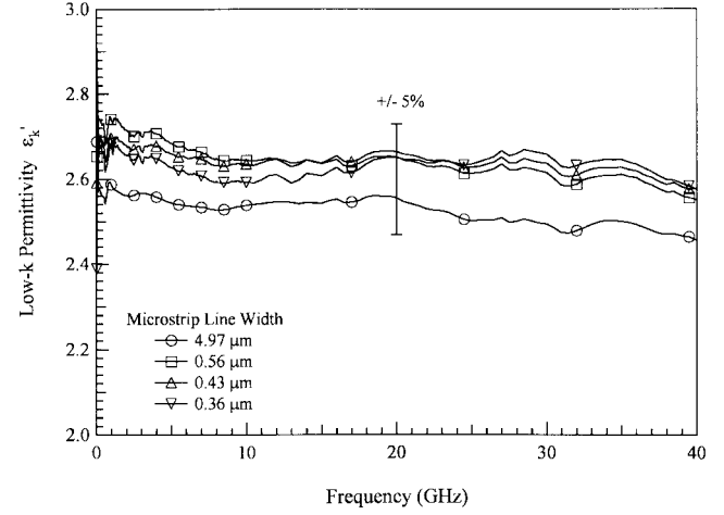
Fig. 10. Relative permittivity of BCB thin film as a function of frequency.
